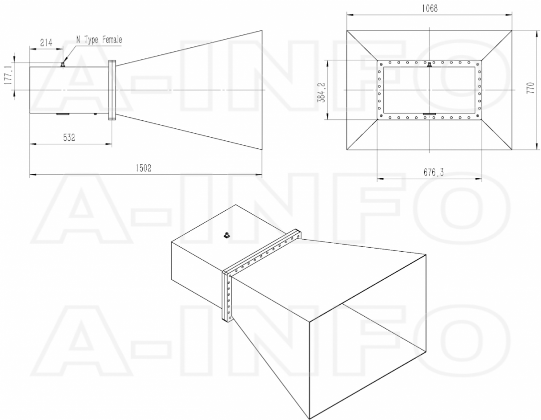
N-Female Output (P/N: LB-2300-10-C-NF)
